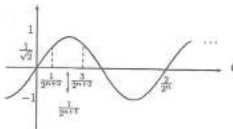
Figura 2.3: f_n(t) = \text{sen } 2^n \pi t
