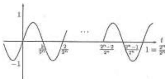
Figura 2.1: \text{sen } 2^n \pi t
